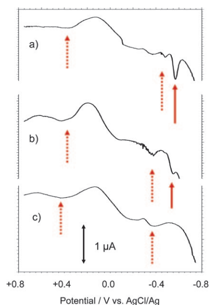
Figure 2. Square-wave voltammograms for samples from a) Acanceh, b) D'zula, and c) Mayapán attached to paraffin-impregnated graphite electrodes immersed into 0.50 M acetic acid/sodium acetate aqueous buffer, pH 4.75. Potential scan initiated at -0.75 V in the positive direction. Potential-step increment 4 mV; square-wave amplitude 25 mV; frequency 5 Hz. Peaks for isatin (solid arrows) and the dehydroindigo/indigo/leucoindigo system (dotted arrows) are marked.
